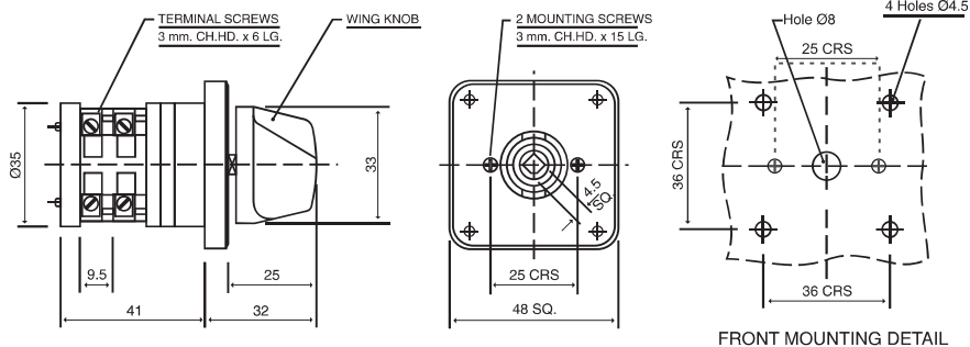
FRONT MOUNTING DETAIL
