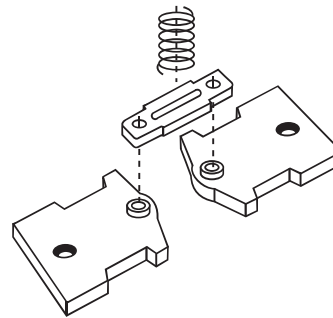
Contact Assembly
