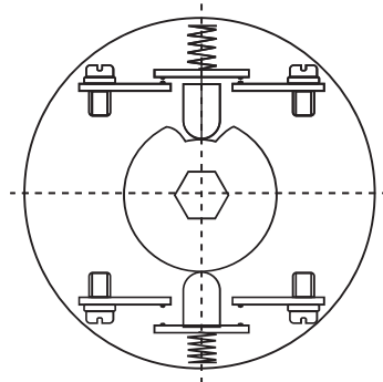
Cam Assembly
